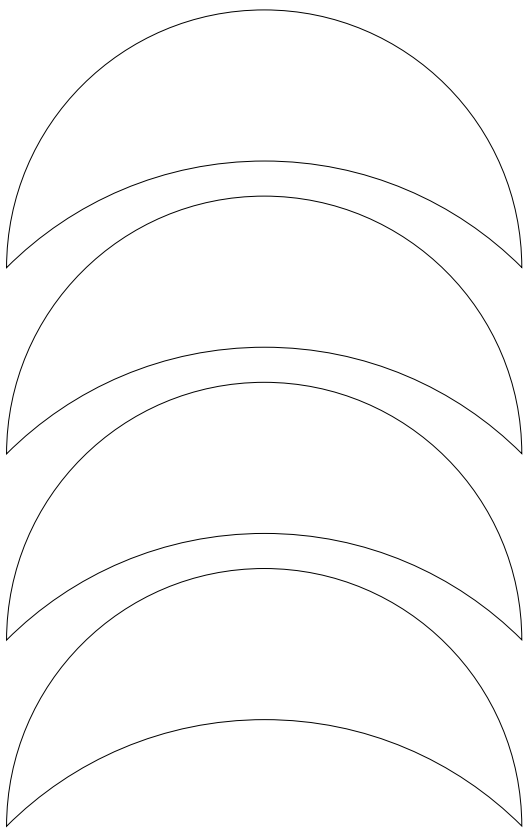
rearmost fairing bulkheads (glue flush with bottom of rocket)
